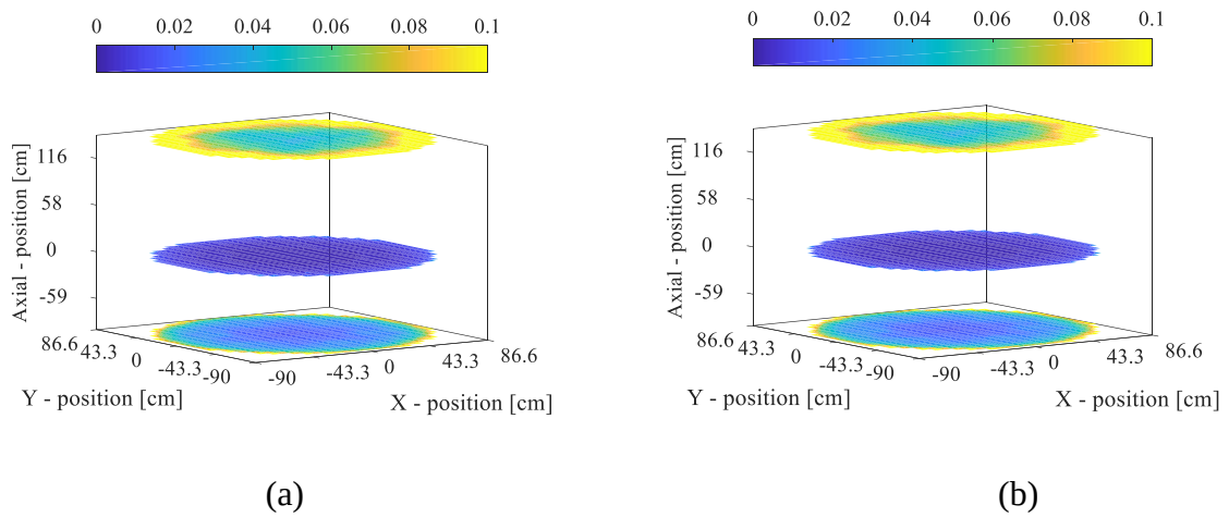
Figure 23 (a) and (b): Color map of radial standard deviations by OpenMC and MCNP respectively.
