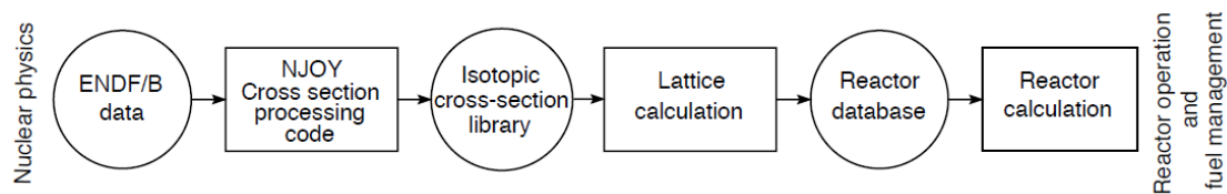
Figure 11: Data library creation steps. (Hebert, 2016)
