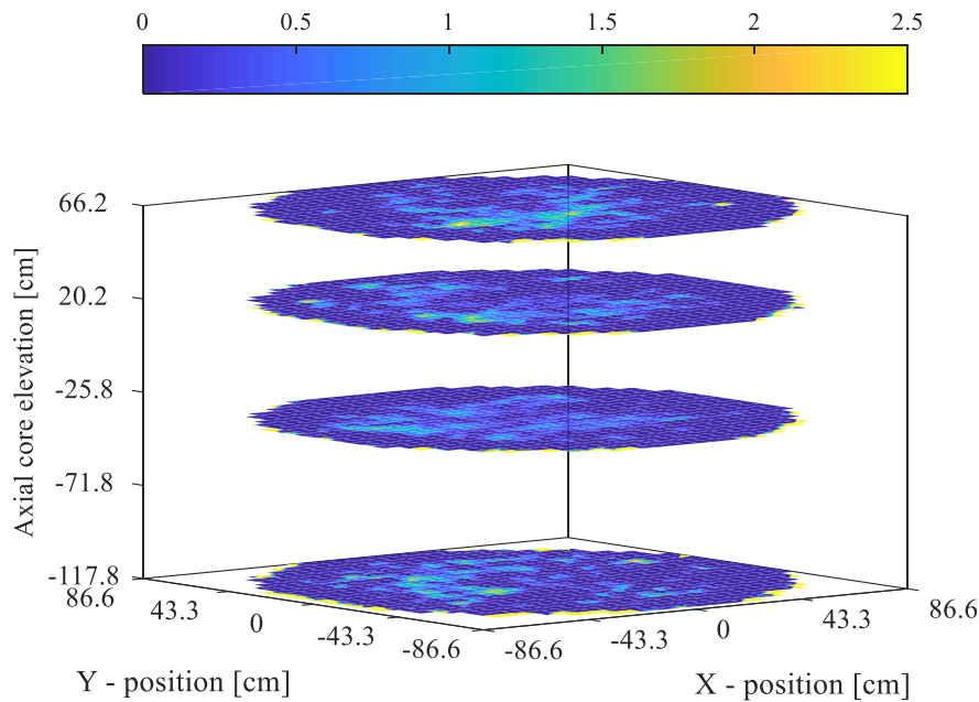
Figure 22 (e): the relative difference between OpenMC and MCNP.
