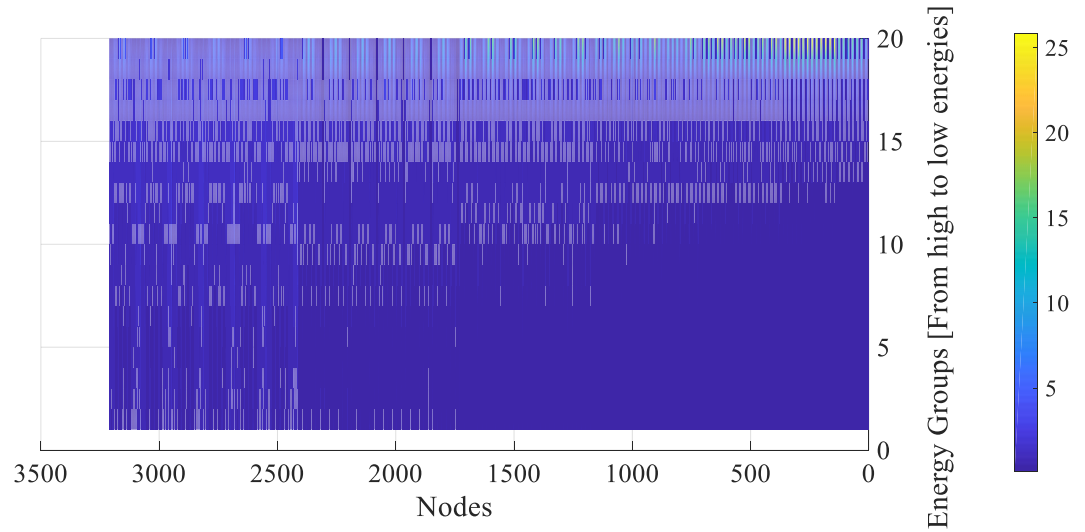
Figure 24: Relative error of the total MGXS.
