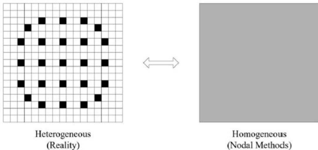
Figure 12: Demonstration of a homogenization at assembly level. (Hall, 2015)
