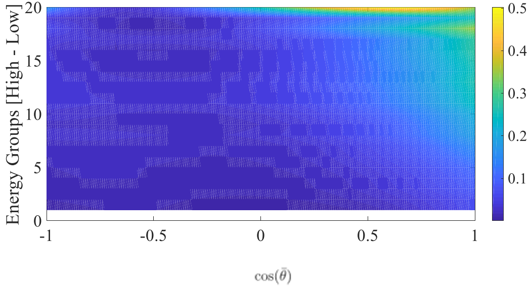
Figure 26: Multi-group scattering cross-section matrix in thermal IPS (water medium).
