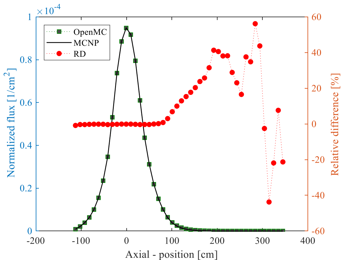
Figure 21: Full core radially averaged volumetrically normalized flux benchmark and the relative difference.
