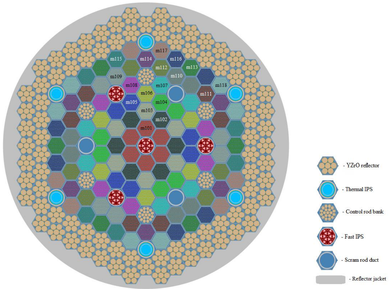
Figure 14: Radial cross-section at fuel mid-span of the MYRRHA 1.6 core model
