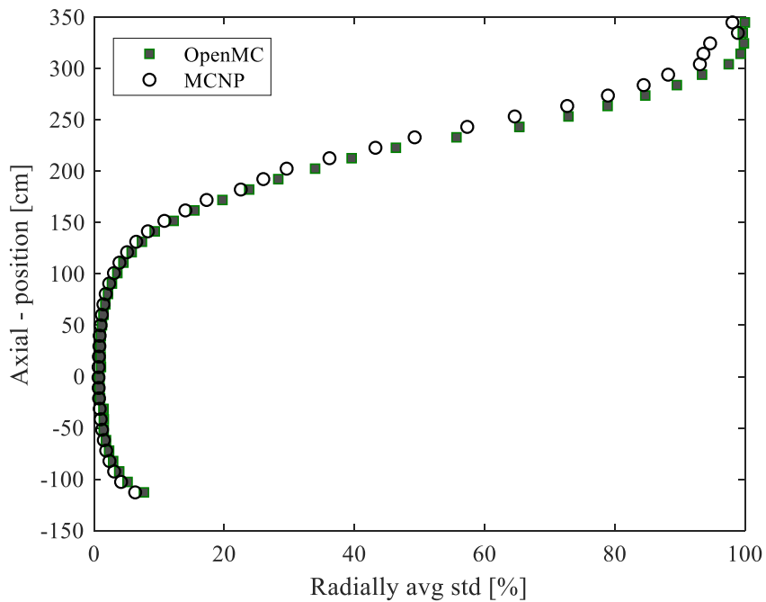
Figure 23 (c): Radially averaged standard deviation.
