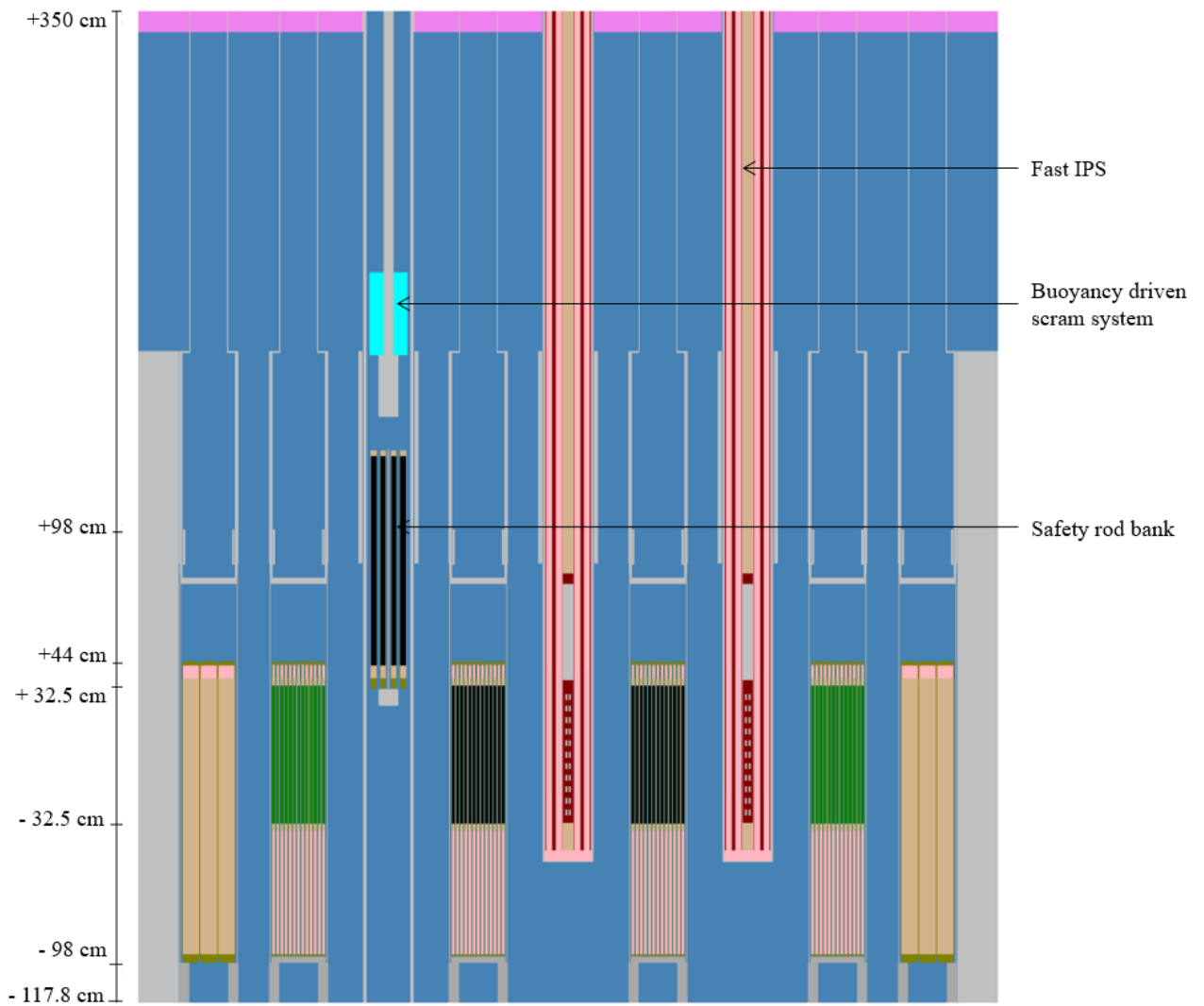
Figure 16: Axial mid-span cross-section view of the MYRRHA 1.6 core model in the xz-axis
