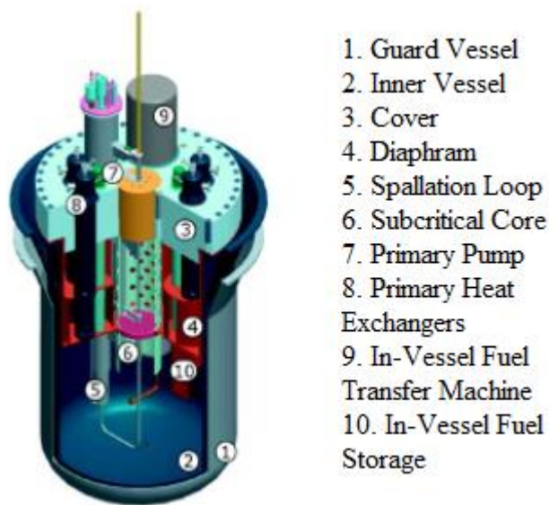
Figure 1: MYRRHA/XT-ADS model. (Abderrahim, et al., 2012)
