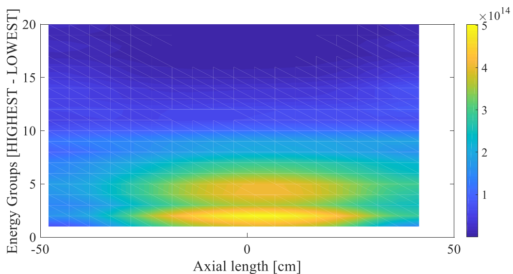
Figure 29: PHISICS flux output in the central IPS
