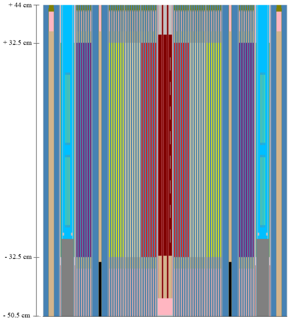
Figure 19: Reduced axial mid-span cross-section view in the yz-axis
