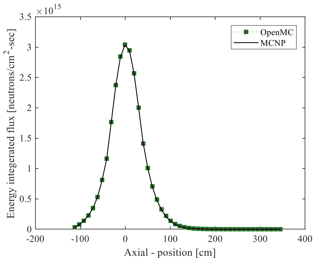
Figure 20: Energy integrated flux at the central channel
