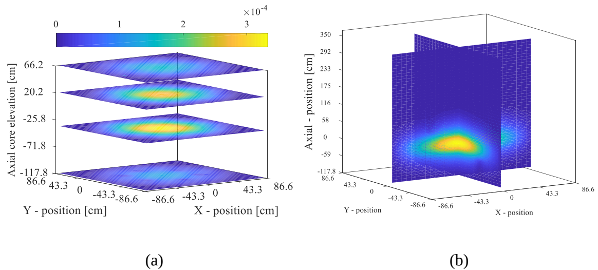
Figure 22 (a) and (b): Color map of radial and axial flux distribution by OpenMC.
