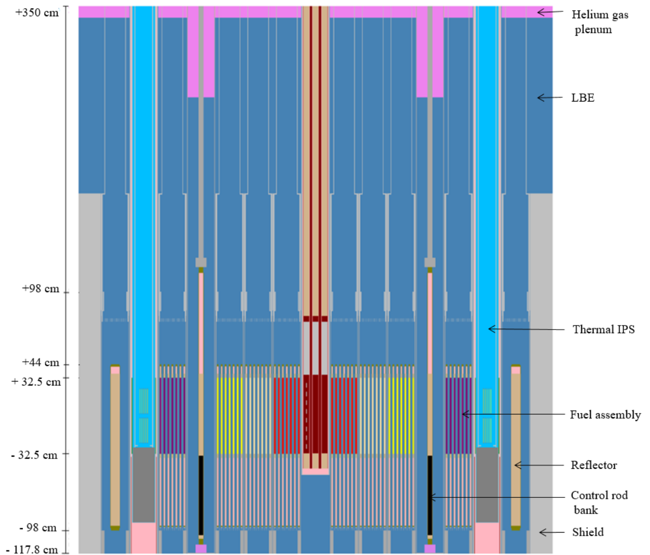
Figure 15: Axial mid-span cross-section view of the MYRRHA 1.6 core model in the yz-axis
