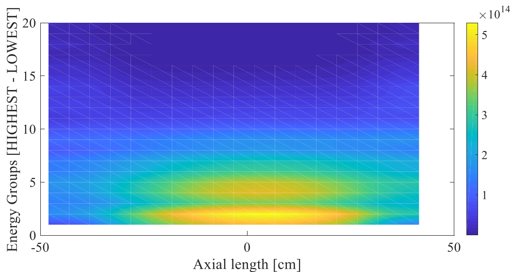
Figure 30: PHISICS flux output in the fuel assembly
