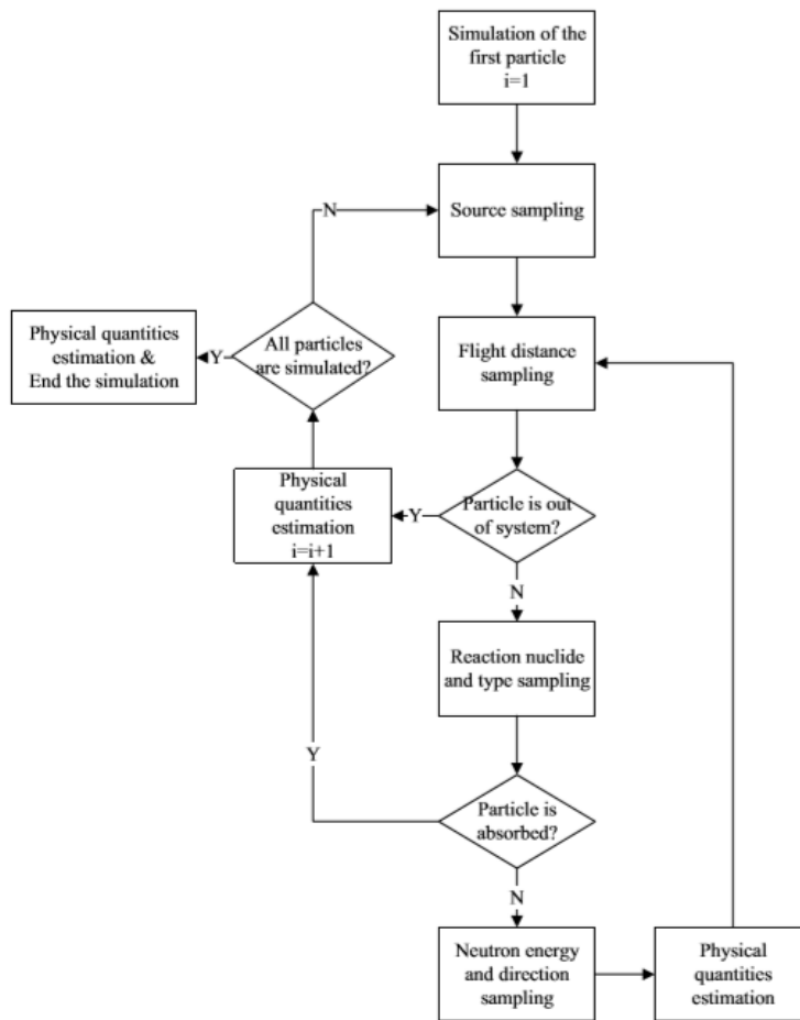
Figure 4: Algorithm of Monte Carlo transport simulation. (Wu, 2019)
