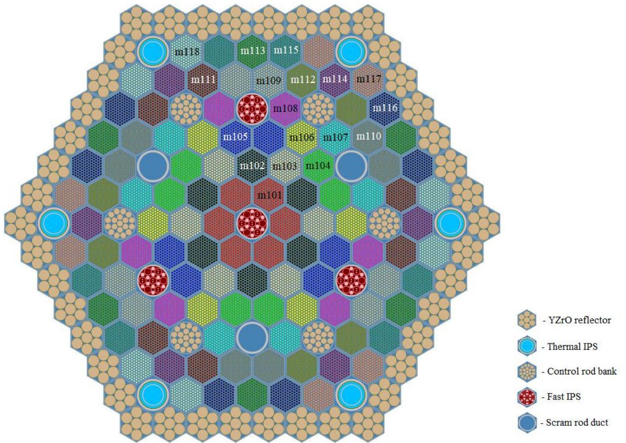
Figure 17: Reduced radial cross-section at fuel mid-span
