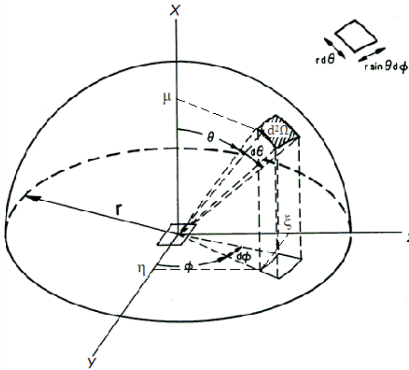
Figure 13: Solid angle. (Howell, 2011)
