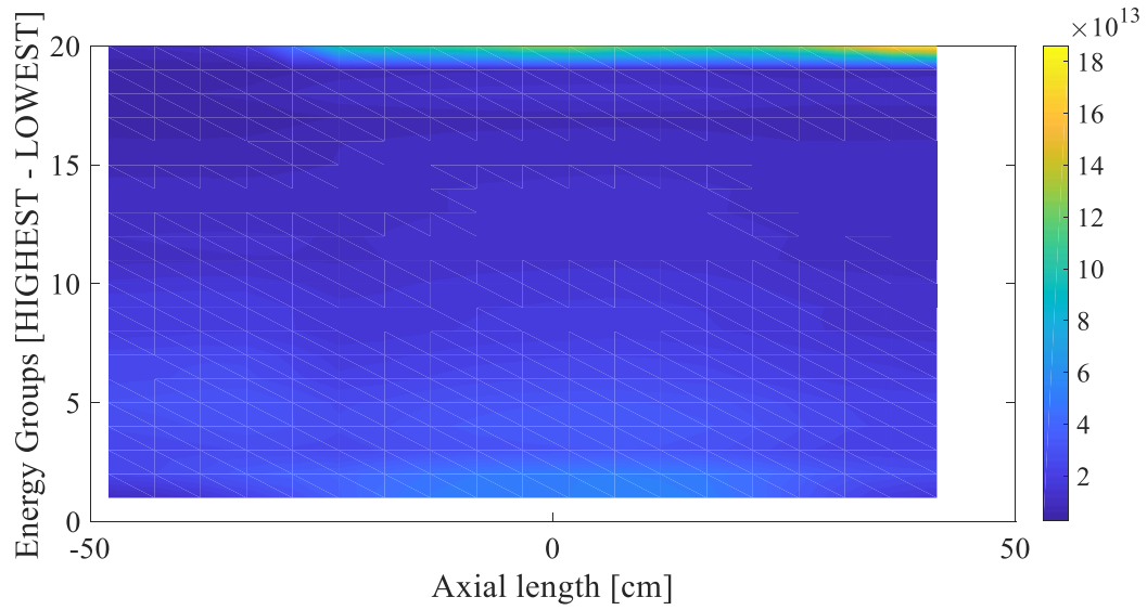
Figure 31: PHISICS flux output in the thermal IPS.
