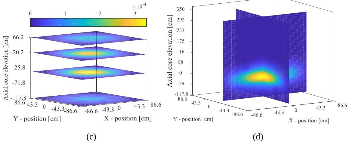
Figure 22 (c) and (d): Color map of radial and axial flux distribution by MCNP.
