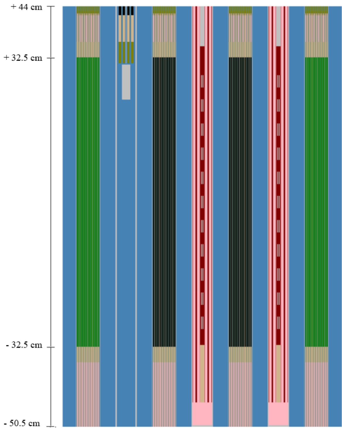
Figure 18: Reduced axial mid-span cross-section view in the xz-axis
