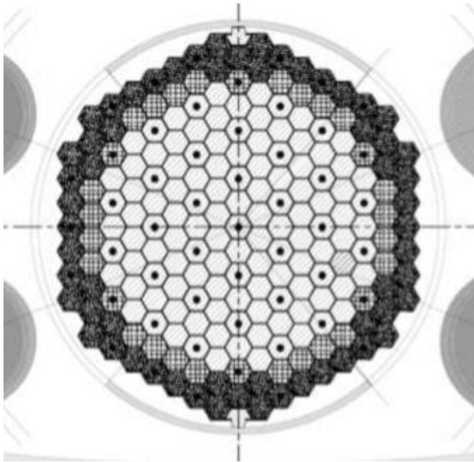
Figure 3: The MYRRHA core lay out. Channels marked with a black dot are accessible from the top during operation. (Malambu & Stankovskiy, 2014)
