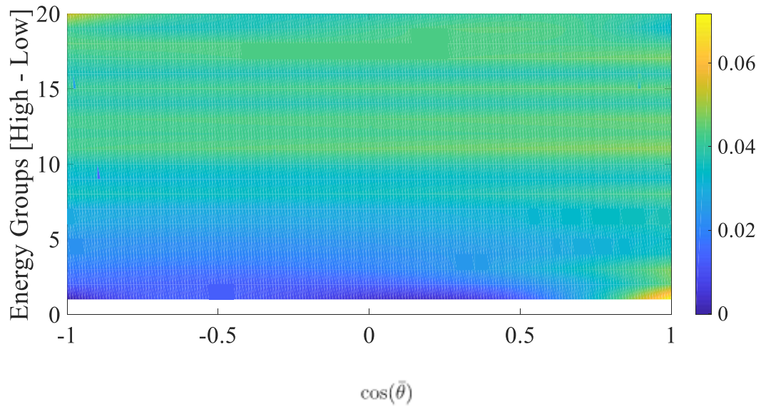
Figure 27: Multi-group scattering cross-section matrix in fuel assembly.
